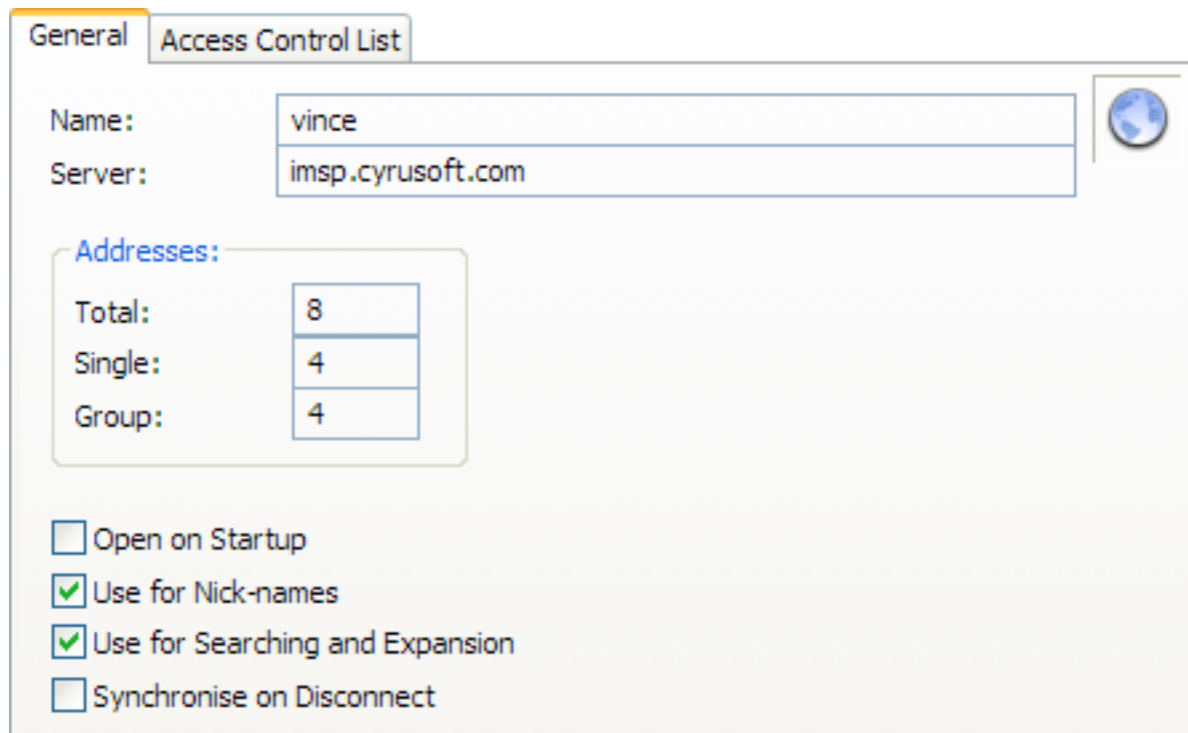
Figure 119 The Address Book Details 'General' panel
