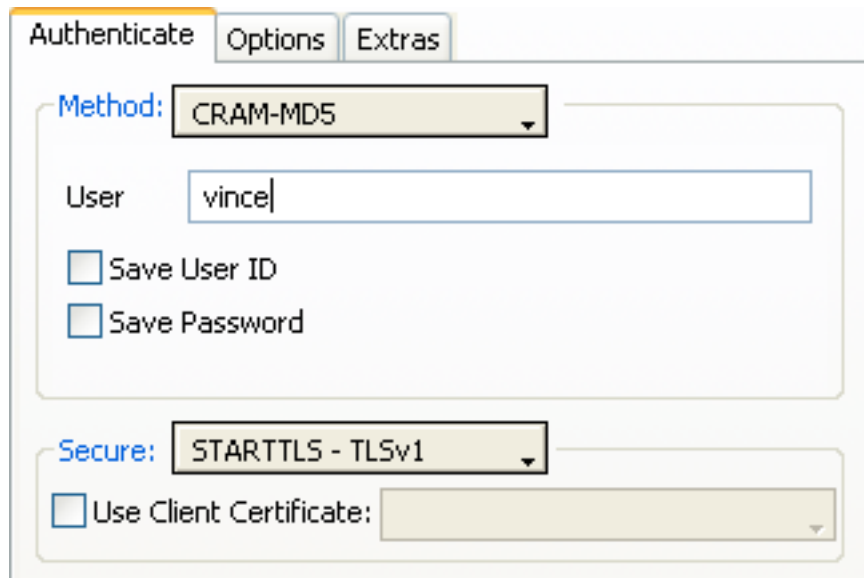
Figure 5 The Authentication tab for authentication methods requiring just a user id and password
