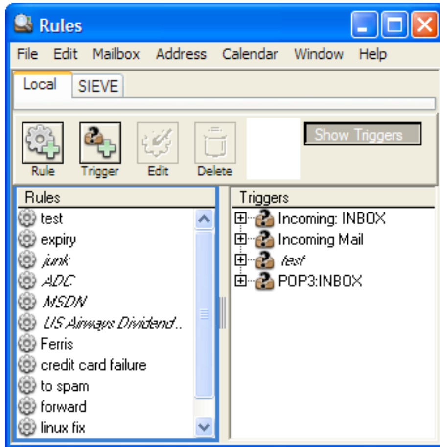
Figure 96 The Rules Manager Window.
