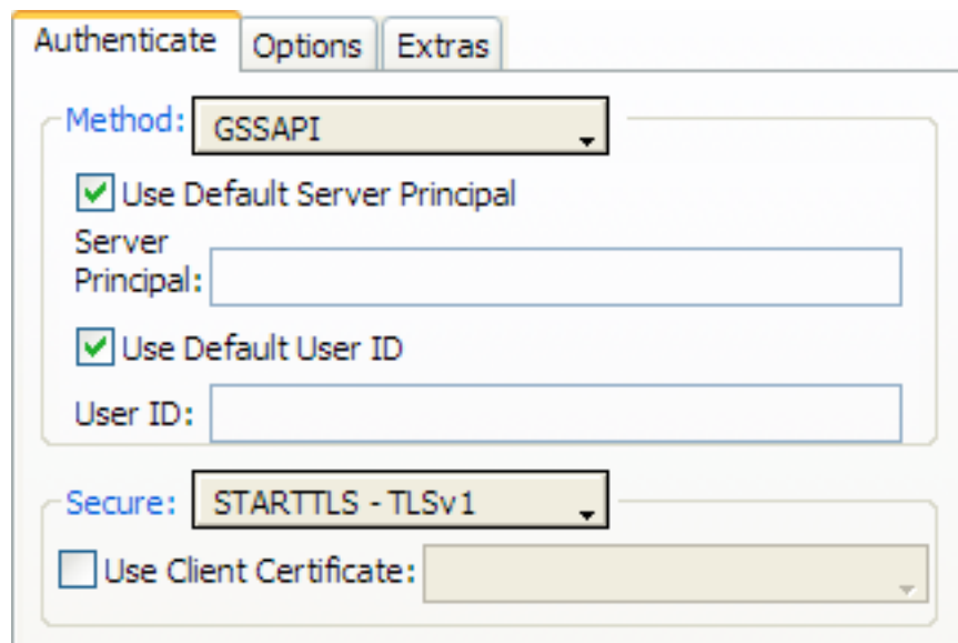
Figure 6 The Authentication panel for Kerberos authentication
