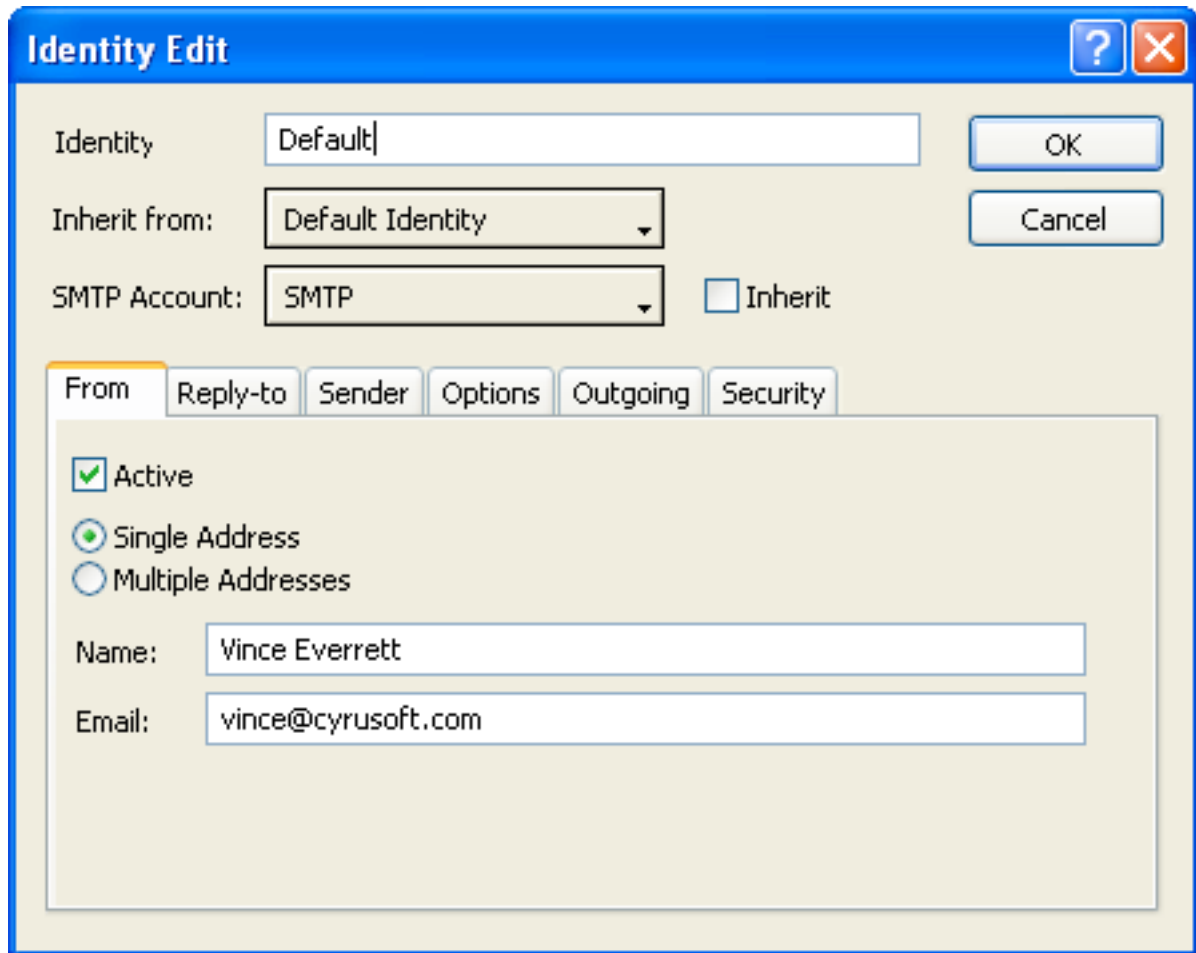
Figure 40 The 'Identity Edit' dialog box
