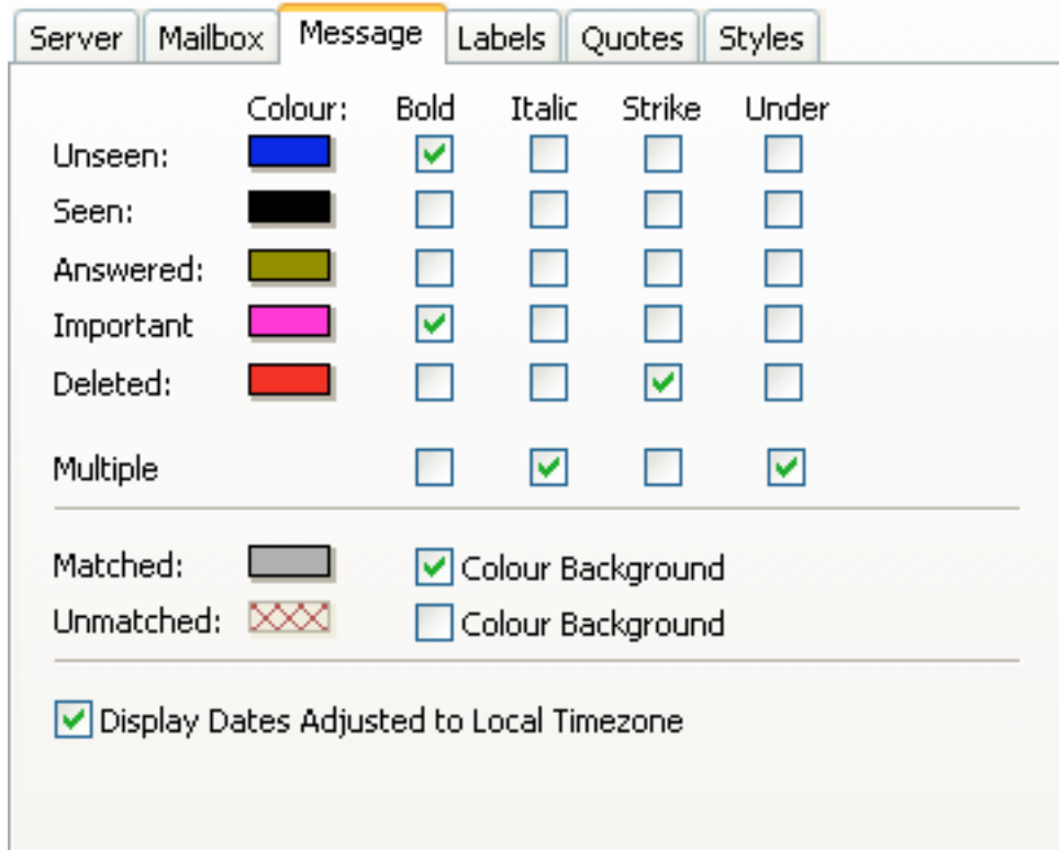
Figure 24 The Message tab in the Display preference panel
